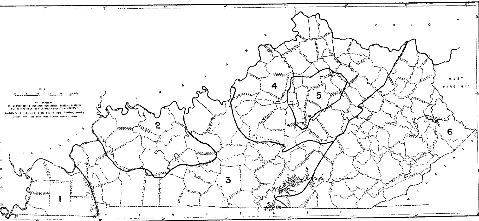
Fig. 1. MAJOR PHYSICAL DIVISIONS OF KENTUCKY
