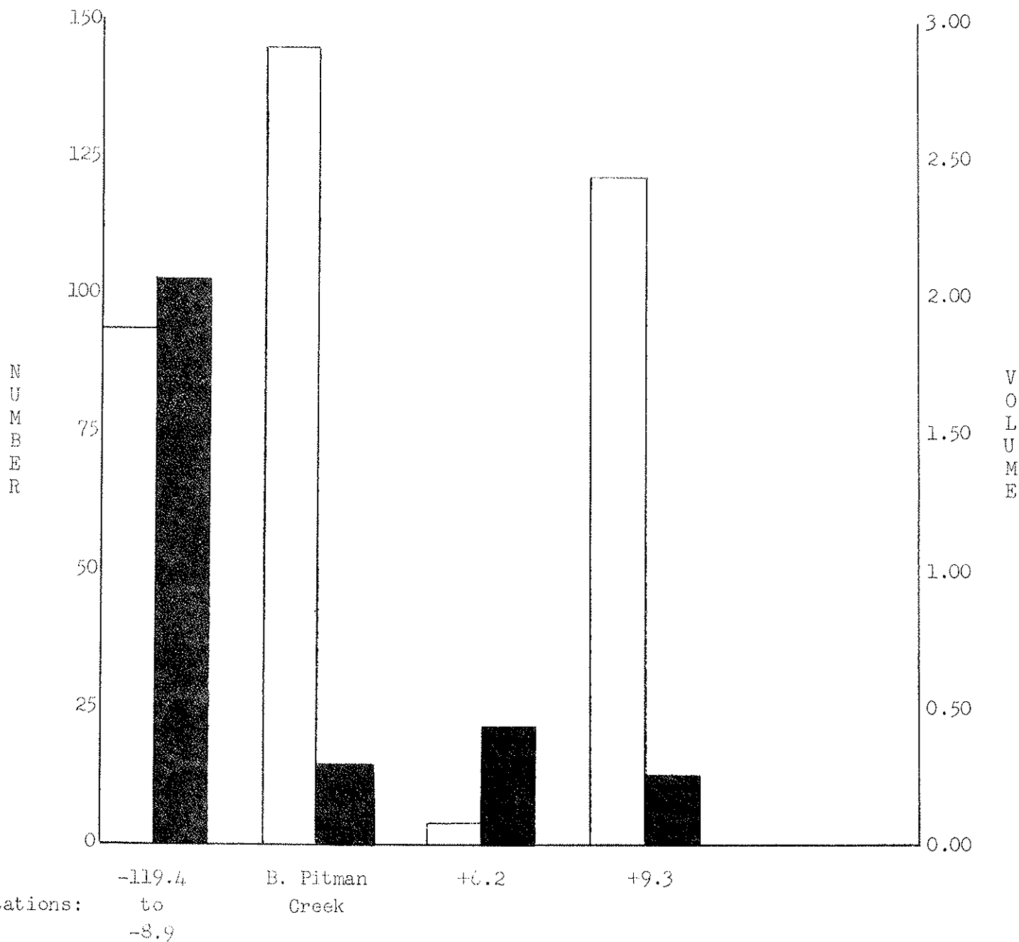
Fig. 1. Mean number and mean volume, per square foot, of macro-invertebrates collected in 1961 from Green River and Big Pitman Creek. Eight stations were located upstream (- = miles above) and two stations were located downstream (+ = miles below) from the oil field pollution. A single station was located on Big Pitman Creek, the prime source of oil field brines.
