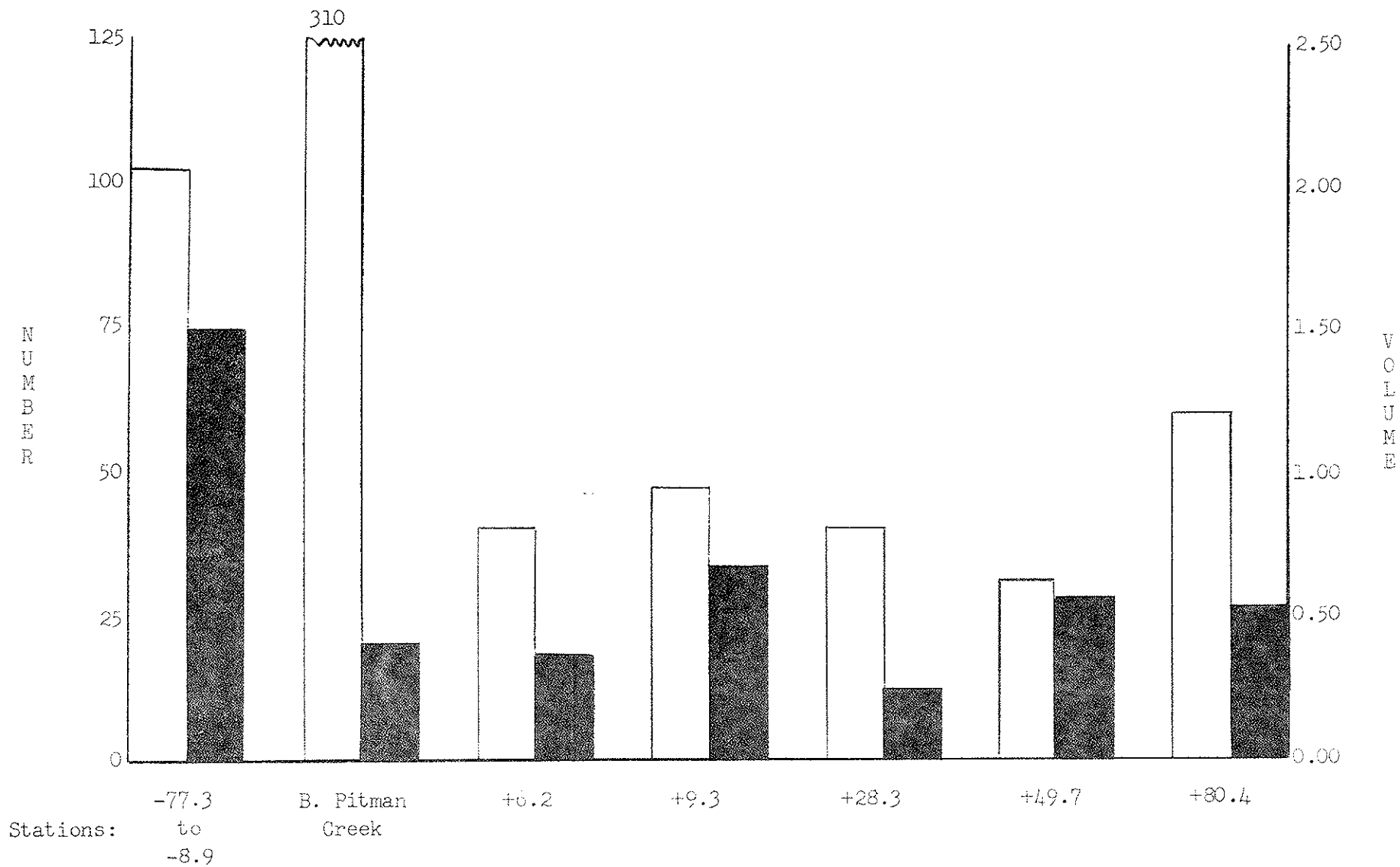
Fig. 5. Mean number and mean volume, per square foot, of macro-invertebrates collected in 1963 from Green River and Big Pitman Creek. Three stations were located upstream (- = miles above) and five stations were located downstream (+ = miles below) from the oil field pollution. A single station was located on Big Pitman Creek, the prime source of oil field brines.
