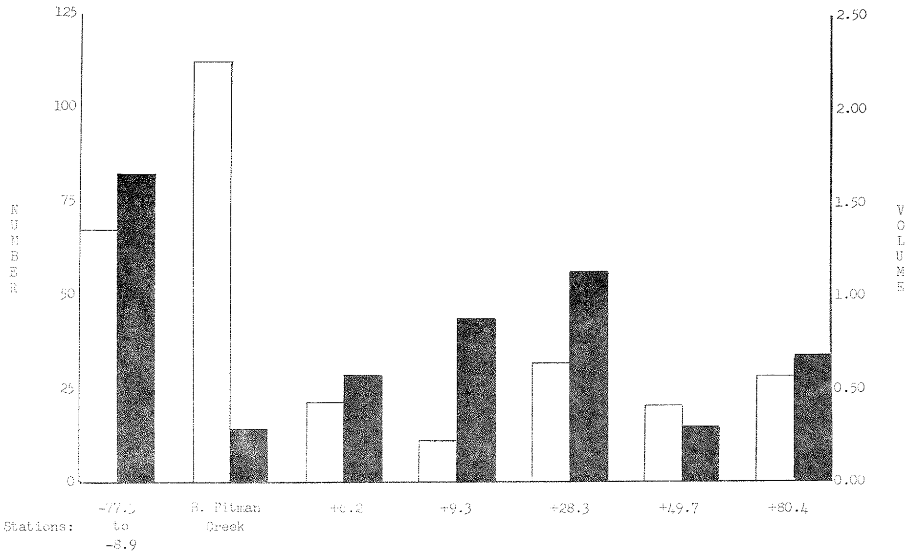
Fig. 4. Mean number and mean volume, per square foot, of macro-invertebrates collected in 1902 from Green River and Big Pitman Creek. Three stations were located upstream (- = miles above) and five stations were located downstream (+ = miles below) from the oil field pollution. A single station was located on Big Pitman Creek, the prime source of oil field brines.
