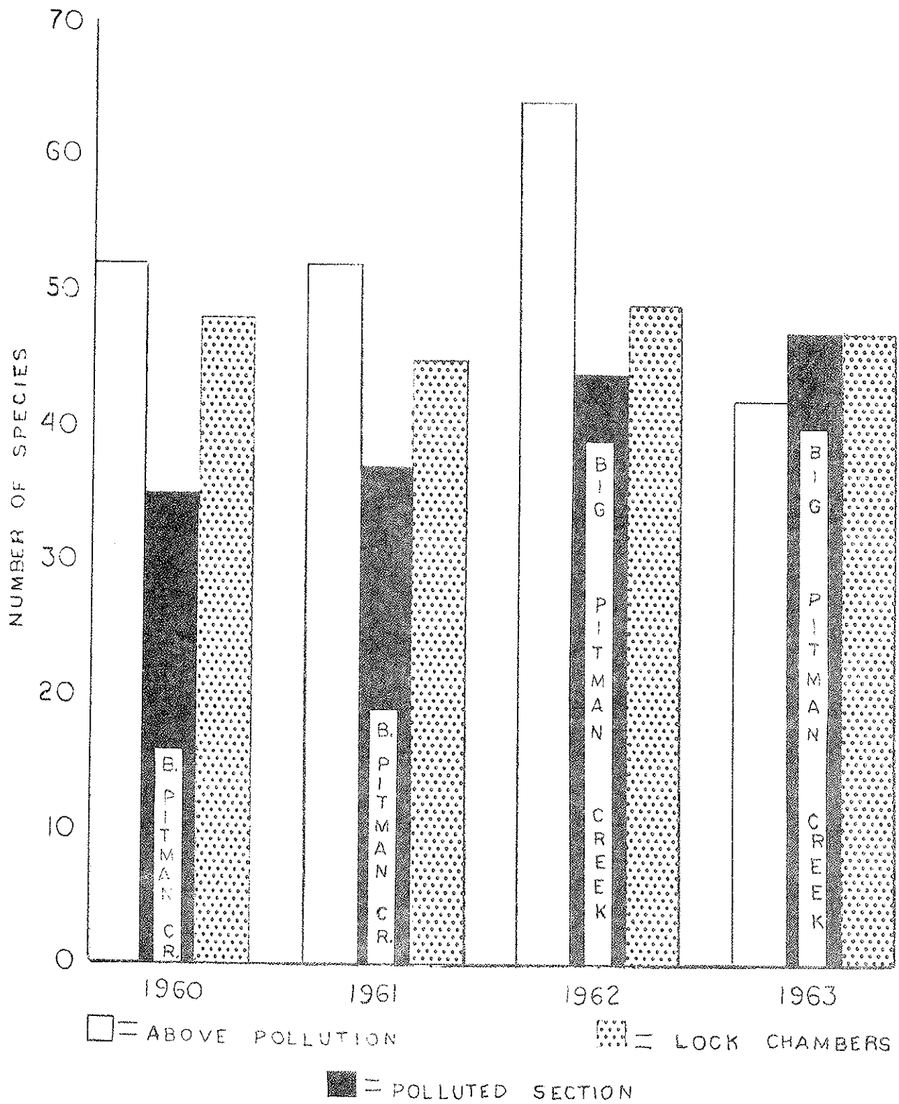
Fig. . The number of species of fishes collected from polluted and non-polluted sections of Green River and from Big Pitman Creek during the years 1960 - 1963. The lock chamber samples were located far enough downstream in the recovery zone to support a normal fish population.
