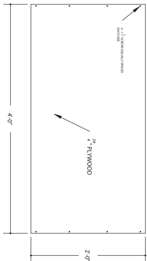
BOW BOX SIDES "A" (2 REQUIRED)
